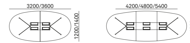
Oval (with top access)
